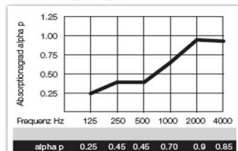
Schallabsorptionsgrad
